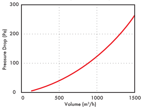
Heat Exchange Resistance Graph
